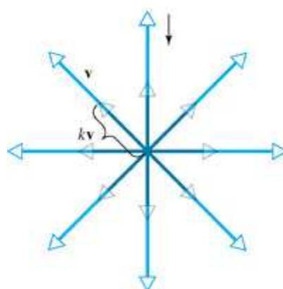
(b) Contraction of V
