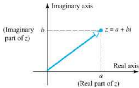
Figure 10.1.3 Argand diagram.
