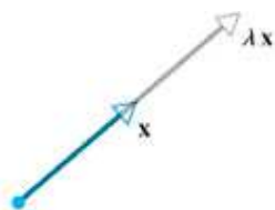
(b) \lambda \geq 1
